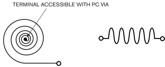
Figure B Spiral and serpentine pc-board patterns sometimes act as high-frequency filters, although they are less effective than ferrite beads.
