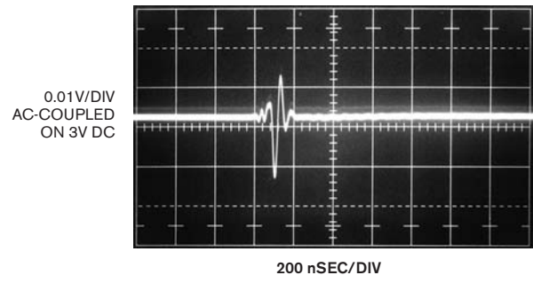
Figure A Spike measured within a continuous coaxial-signal path displays moderate disturbance and ringing after the main event.
