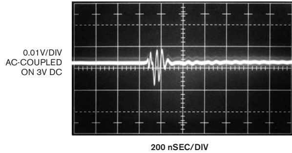
Figure B Introducing a 3-in., noncoaxial ground connection causes pronounced signal distortion and postevent ringing.
