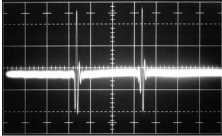
Figure D A low-noise preamplifier and strictly enforced coaxial signal path yield Figure 12's 900-mV p-p presentation. The trace's baseline thickening represents the preamplifier's noise floor.
