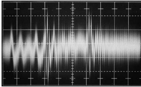
Figure E A 2-in. noncoaxial ground connection at the measurement site violates the coaxial regime, resulting in complete corruption of the waveform presentation.
