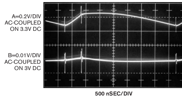
Figure 8 C_{IN} of 1 \mu\text{F} and C_{OUT} of 33 \mu\text{F} result in the same trace assignments as Figure 7. Output ripple decreases fivefold, but spikes remain. Spike rise time appears unchanged.
