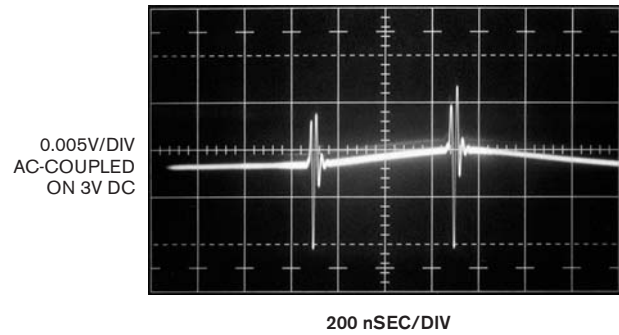
Figure 9 A time and amplitude expansion of Figure 8's output trace permits higher resolution study of spike characteristics. (The trace center-screen area is intensified for photographic clarity.)
