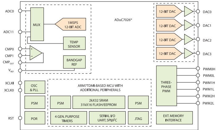
Figure 1 Precision analogue peripherals suit the AD \mu C 70xx family to sensor interface applications.
