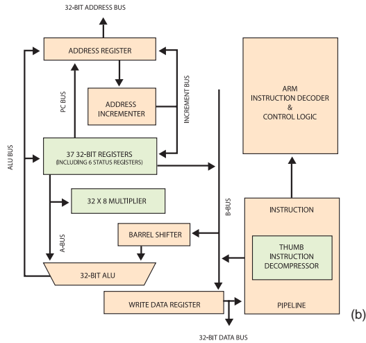
Figure A The ARM7TDMI's debug facilities include embedded in-circuit emulation (a). Its core includes a multiplier and barrel shifter built around a 37-entry register file (b).
