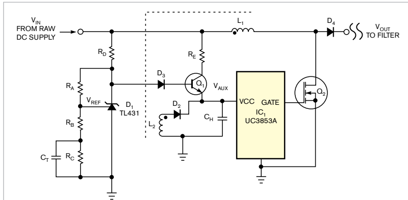
Figure 2 In this augmented bootstrap circuit, transistor Q_1 delivers a robust initial pulse of current to capacitor C_H , ensuring faster start-up and power delivery.
