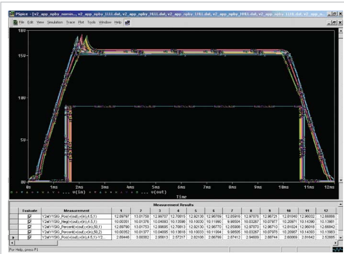
Figure 1 On-screen waveforms represent inputs and outputs for multiple simulation passes.
