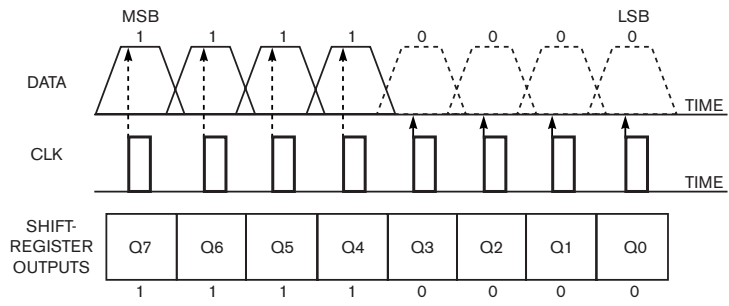
Figure 2 The sample timing diagram illustrates the loading of $F0 byte into an external shift register.
