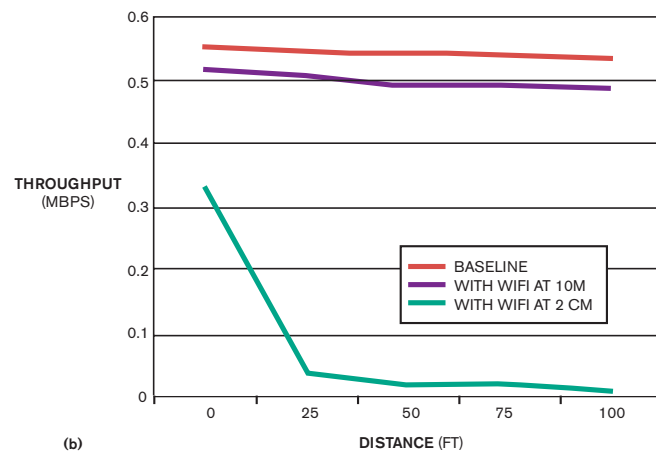
Figure 1 The data rates of WiFi suffer whenever Bluetooth is operating, especially if Bluetooth is close by (a). Bluetooth, however, sees little degradation unless the WiFi transmitter is close (b, courtesy Texas Instruments).
