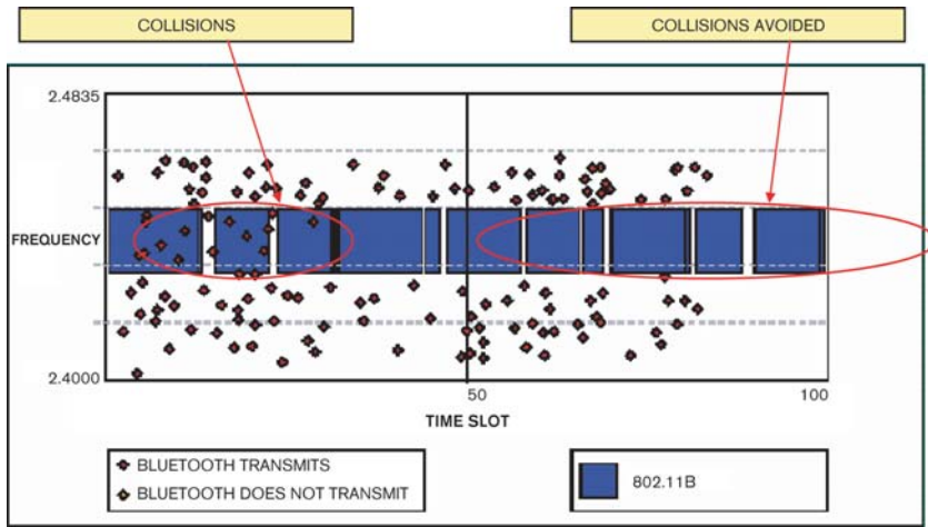
Figure 2 Adaptive frequency hopping uses features available in Bluetooth 1.2 to restrict transmissions on channels on which another transmitter is occupying a fixed bandwidth. The result is fewer collisions and greater throughput (courtesy STMicroelectronics).
