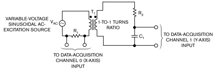
Figure 1 The test fixture for a basic hysteresis-loop analyzer requires few components.
