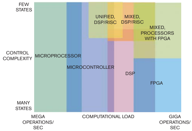
Figure A A conceptual mapping shows how the sweet spots of processing architectures can complement each other to cover the range of an application's processing requirements (assistance from Gary Banta, chief executive officer of Stretch).
