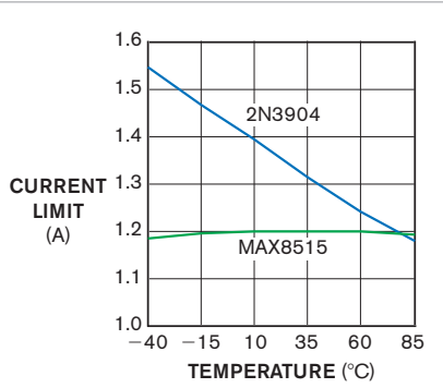
Figure 3 Output-current-versus-temperature plots for the circuits of figures 1 and 2 show improved accuracy for the shunt-regulated circuit (bottom trace) over the discrete-transistor version (top trace).
