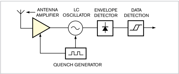
Figure 2 The super-regenerative receiver is considerably simpler than a superheterodyne circuit.
