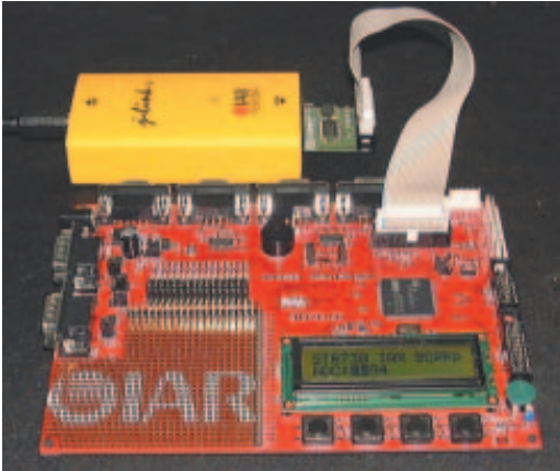
Figure 2 A small adapter connects the 3.3V J-Link emulator to the 5V silicon on IAR's STR730 board.
