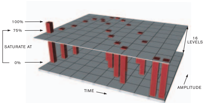
Figure 1 Analog-persistence mode maps frequency of occurrence into intensity or color variations on each pixel of the display simulating the phosphor response of an analog oscilloscope (courtesy LeCroy).
