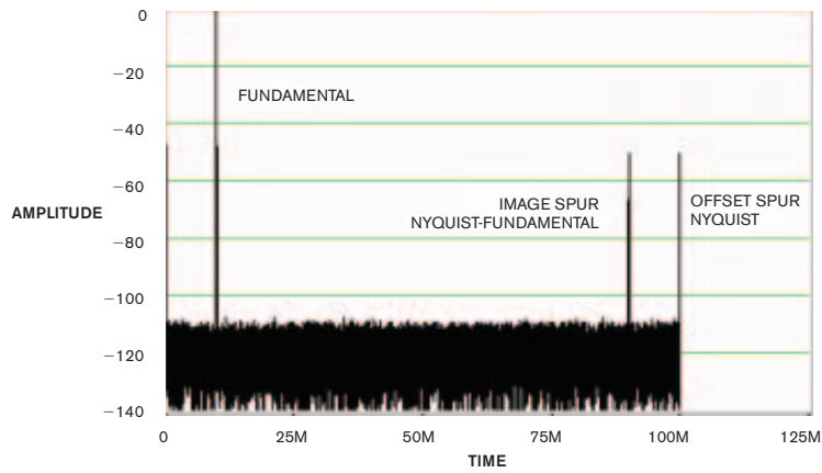
Figure A Time-interleaved sampling of two 12-bit, 100M-sample/sec ADCs results in an effective sampling rate of 200M samples/sec. Gain and phase mismatch between the ADCs results in the image spur , and the offset mismatch between the ADCs results in the offset spur .
