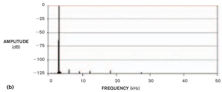
Figure B These FFT plots show what happens when you apply a pure sine wave to a 6-bit delta-sigma ADC before linearization (a) and afterward (b).
