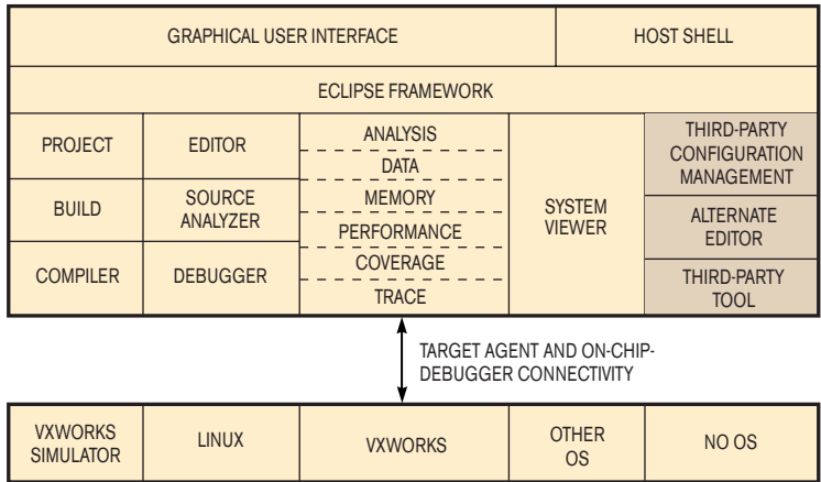
Figure 1 The Wind River Workbench suite integrates Linux and VxWorks design tools into the open-source Eclipse integrated development environment.
