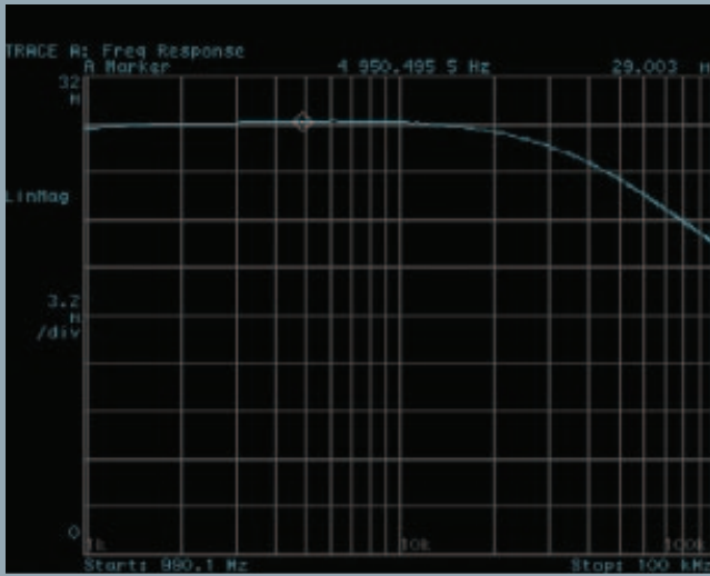
Figure G In this gain-versus-frequency plot of the circuit in Figure C, the midband flat gain is 0.0290. This gain rolls off to 0.0212 at 100 kHz, indicating a relative gain of 0.73 at 100 kHz.
