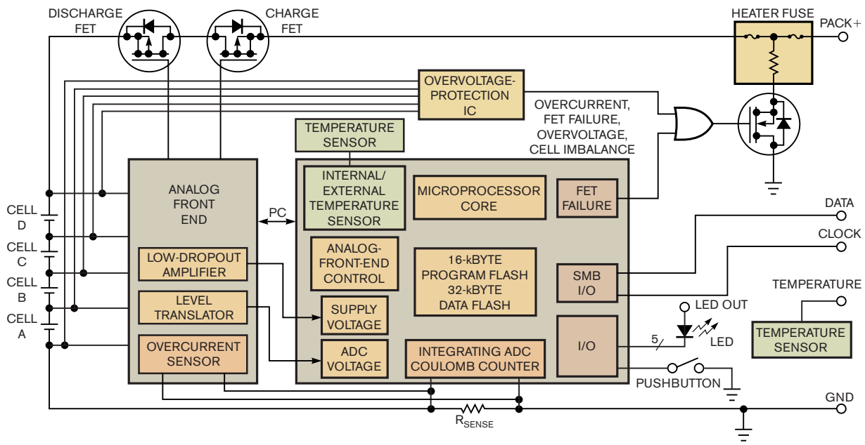
Figure 3 A typical notebook-computer battery-pack circuit uses multiple cells.
