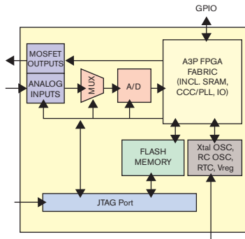
Figure 1 With analogue inputs, flash memory and MOSFET driver outputs, Actel's Fusion PSC can extend the single-chip concept to cover even more of a control system.
