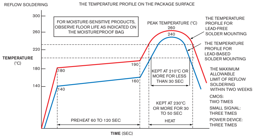
Figure 1 The surface temperature for packages soldered with lead-free materials can be as much as 40°C greater than those packages using leaded solder. This temperature difference can impact board layout and materials handling (courtesy Toshiba America Electronic Components).
