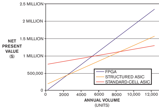
Figure 3 At volumes of less than 1500 parts per year, such as might be the case for an avionics-control chip, an FPGA may be your best bet.
