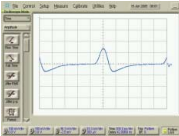
Figure 4 The impulse response shows some pulse broadening due to the limited bandwidth of the channel.
