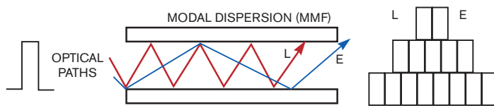
Figure 2 Imperfections in fiber and continued degradation over time cause modes to propagate through the fiber at different speeds. This situation leads to dispersion and potential overlapping of light.
