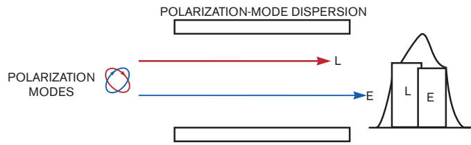
Figure 3 PMD causes a single pulse to spread at the far end because of the delayed arrival of the two perpendicular polarization modes within the fiber.
