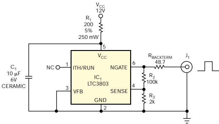
Figure 1 Switching-regulator-controller IC_1 delivers pulses with 1.5-nsec rise and fall times into a 50 \Omega load.
