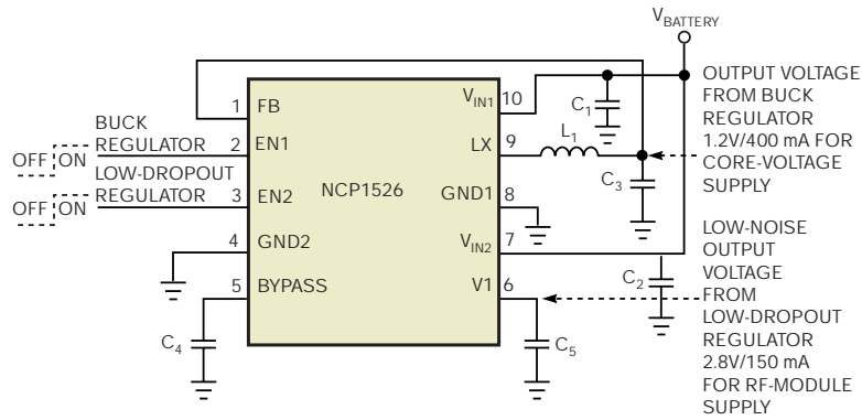
Figure 2 Vendors are beginning to introduce integrated power ICs with both buck and low-noise, low-dropout regulators.
