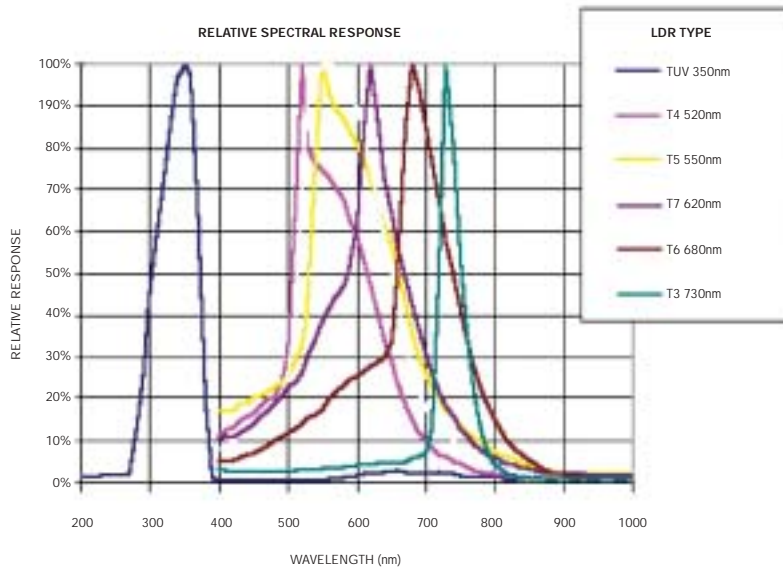
Figure 2 Alternative compounds give Silonex' light-dependent resistors peak responses that span ultraviolet to near-infrared.
