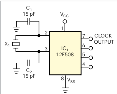
Figure 1 Delivering a fixed clock frequency, this preprogrammed oscillator uses few components.
