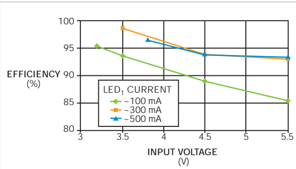
Figure 2 Circuit efficiency versus input voltage shows an increase in efficiency for increasing LED current and decreasing input voltage.
