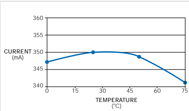
Figure 3 Current through the LED varies less than 3% over an operating-temperature range of 0 to 75°C.
