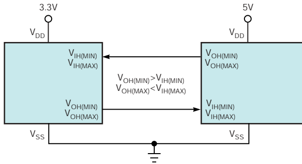
Figure 1 In a two-rail system, devices with different logic levels must communicate.
