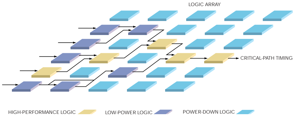
Figure 3 Altera's Stratix III assigns high-performance logic elements to critical paths and low-power logic elements to noncritical paths, and it powers down unused logic elements to reduce leakage.
