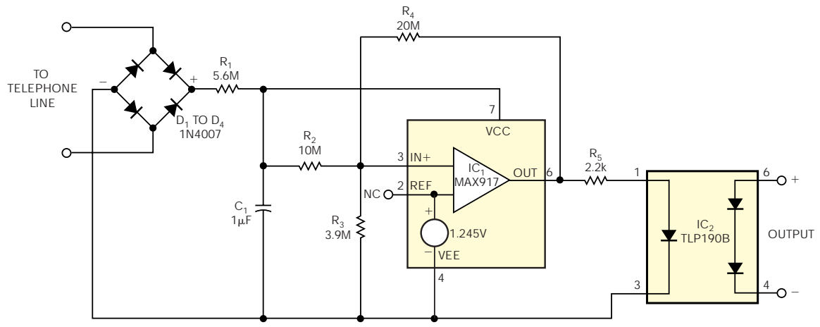
Figure 1 Drawing minuscule amounts of power from a telephone line, this isolated-output circuit indicates whether the line is in use.
