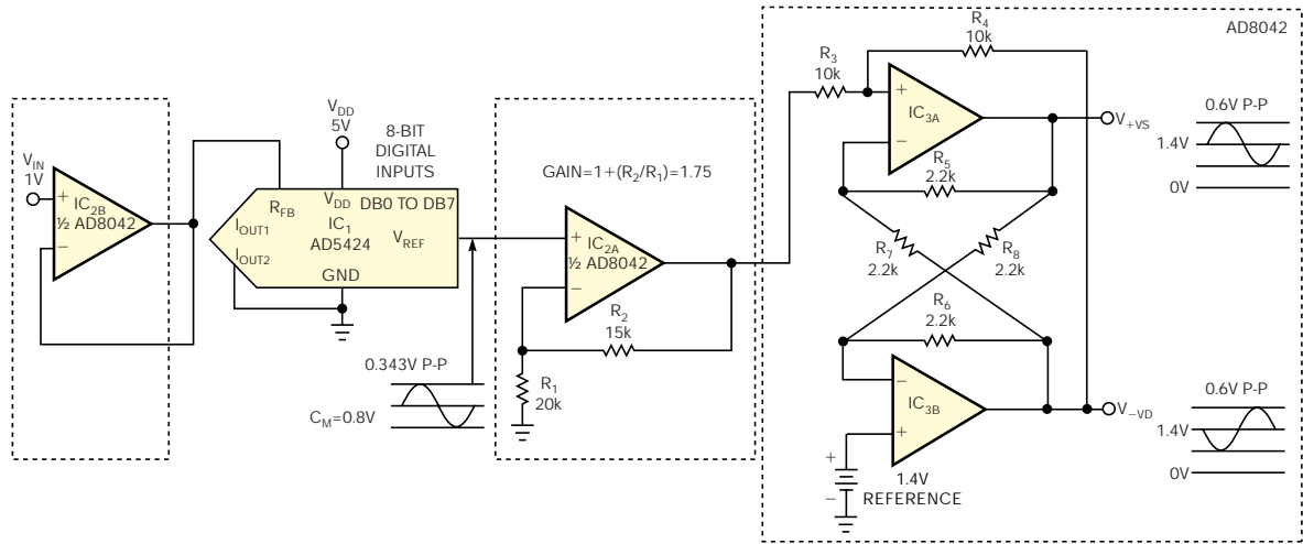
Figure 2 In this configuration, a positive reference voltage produces a positive output voltage.
