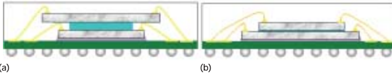
Figure 4 When the performance of the smaller die is important, the same-size stacking option (a) gives better performance than the pyramid-stacking option (b).
