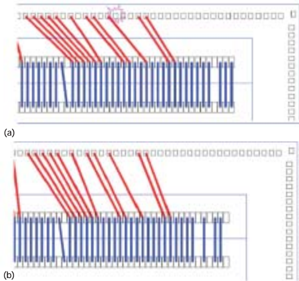
Figure 2 You can avoid a shorted wire (a) by shifting relative die location (b).
