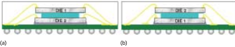
(a) (b) Figure 5 Die 1 requires significantly fewer wires than Die 2. Placing Die 2 on the bottom (a) results in smaller bond-finger pitch, but placing Die 1 on the bottom results in a larger bond-finger pitch (b).
