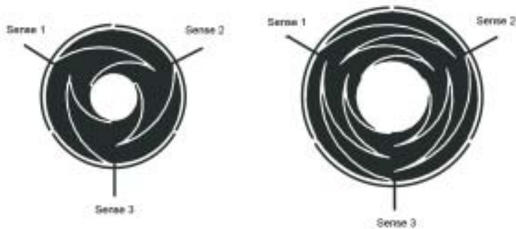
Figure 4 Quantum's wheel sensors can use a 3-terminal interleaved metal structure to re-solve 128 points.
