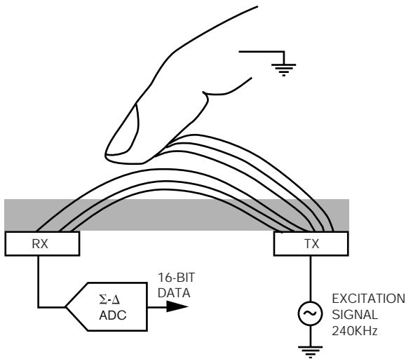
Figure 1 Shunt capacitance disturbs the sense field that the AD7142 creates.
