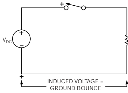
Figure 2 When the formerly closed switch in this simple circuit opens, the magnetic flux goes to zero, inducing a voltage along the circuit.
