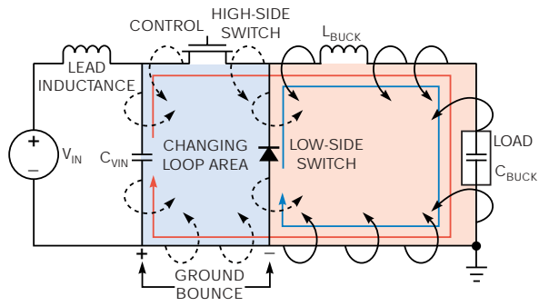
Figure 6 A switching power semiconductor replaces the simplified switch of Figure 5.
