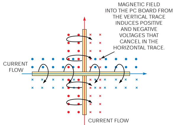
Figure A The magnetic field from the vertical trace induces positive and negative voltages that cancel in the horizontal trace.
