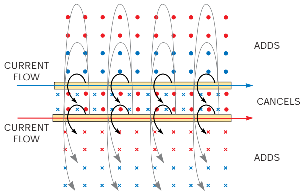
Figure B Wide pc-board traces have less inductance than narrow traces.
