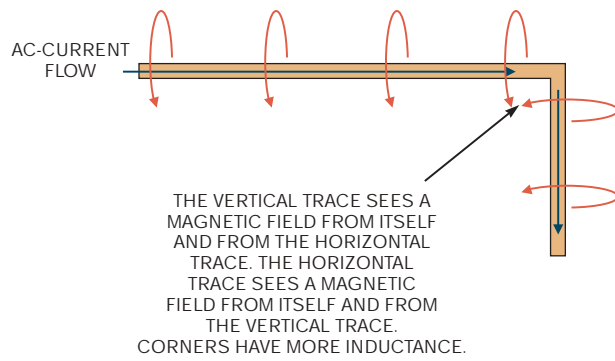
Figure D Both the vertical and horizontal traces see a magnetic field from themselves as well as from the perpendicular trace.
