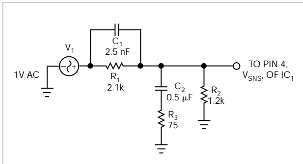
Figure 4 A few passive components supplement R_1 and R_2 and stabilize the circuit for use with a ceramic-dielectric output-filter capacitor.
